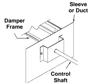
Outboard Shaft Support Bracket
