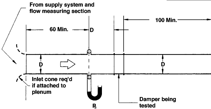
AMCA STANDARD 500 FIGURE 5.3 DAMPER TEST SETUP WITH INLET AND OUTLET DUCTS
